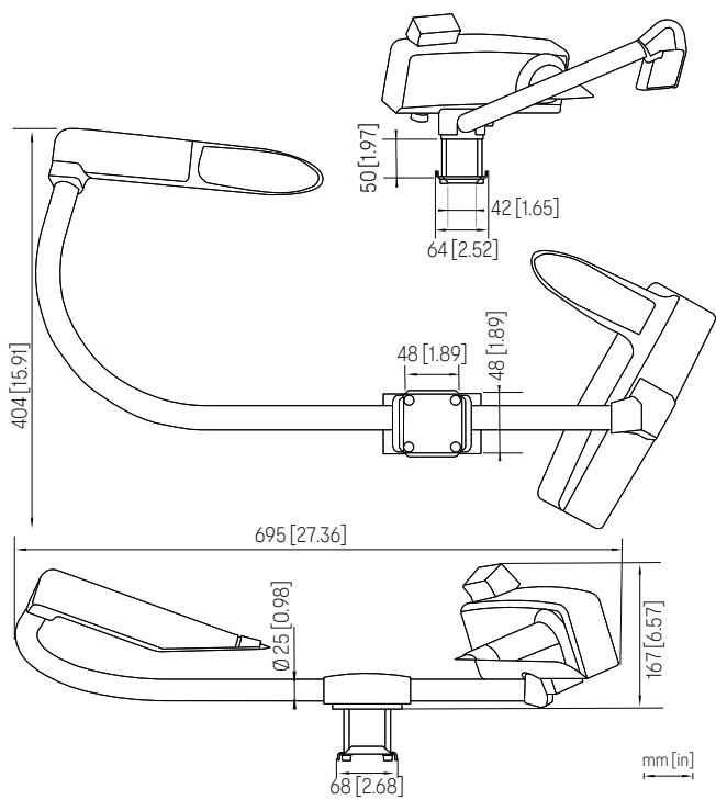
PWD22 dimensions
