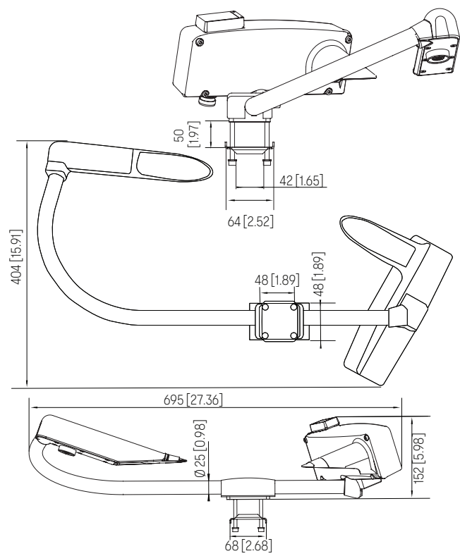
PWD12 dimensions
