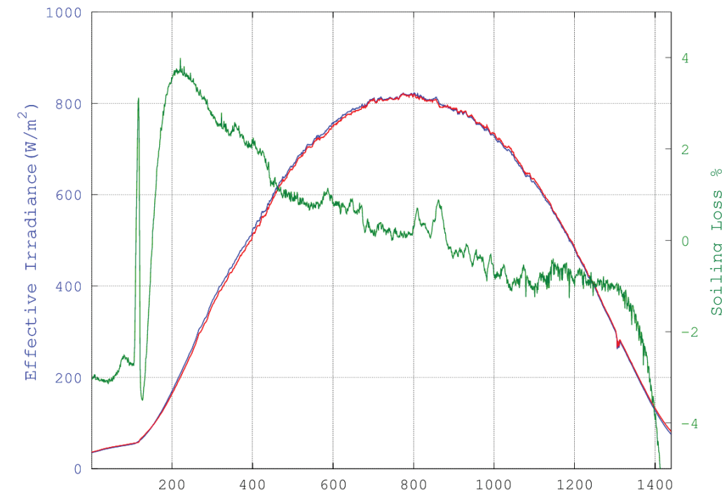
Figure 1: Effective irradiance as calculated from the short-circuit current of the PV modules on a clear-sky day. The green curve shows daily soiling loss.
