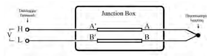
FIGURE 87: Diagram of a Thermocouple Junction Box
