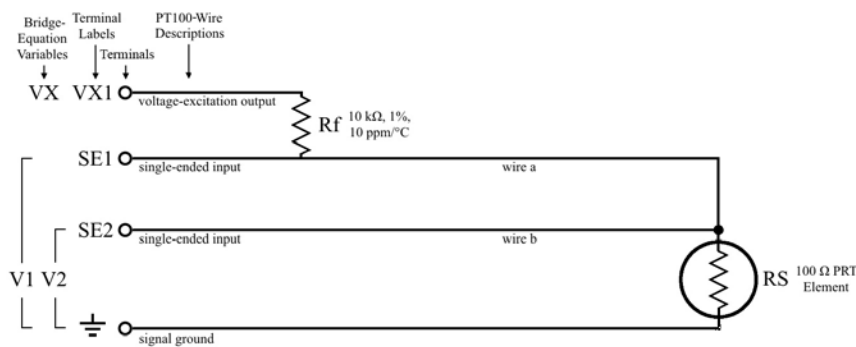
FIGURE 68: PT100 BrHalf3W() Three-Wire Half-Bridge Schematic
