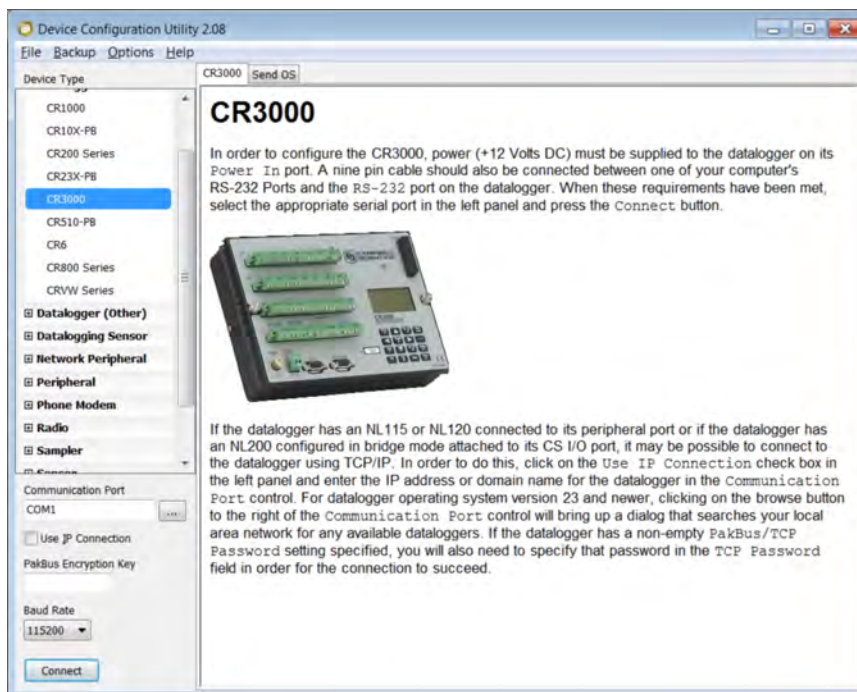
FIGURE 35: Device Configuration Utility (DevConfig)
