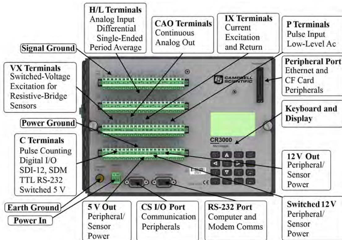
FIGURE 1: Wiring Panel
