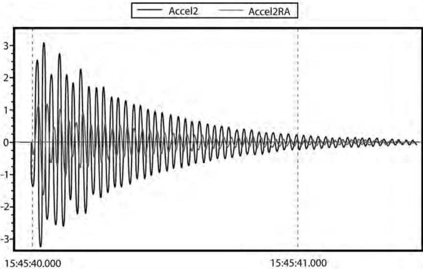
FIGURE 43: Running-Average Signal Attenuation
