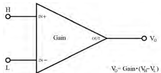
FIGURE 90: Programmable Gain Input Amplifier (PGIA): H to V+, L to V–, VH to V+, VL to V– correspond to text.
