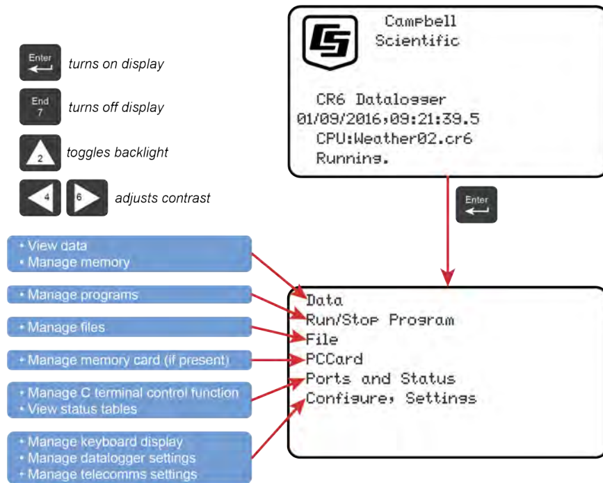
FIGURE 109: Keyboard and Display: Navigation
