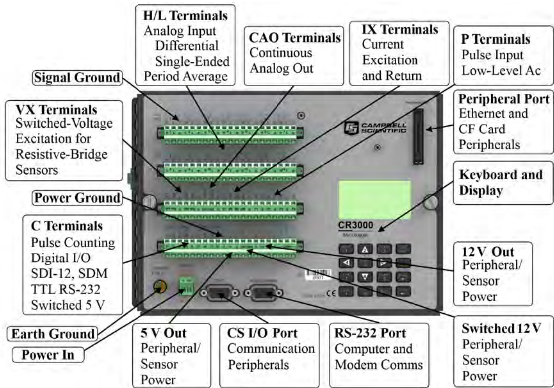
FIGURE 17: Wiring Panel
