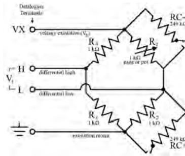
FIGURE 61: Quarter-Bridge Strain Gage with RC Resistor Shunt
