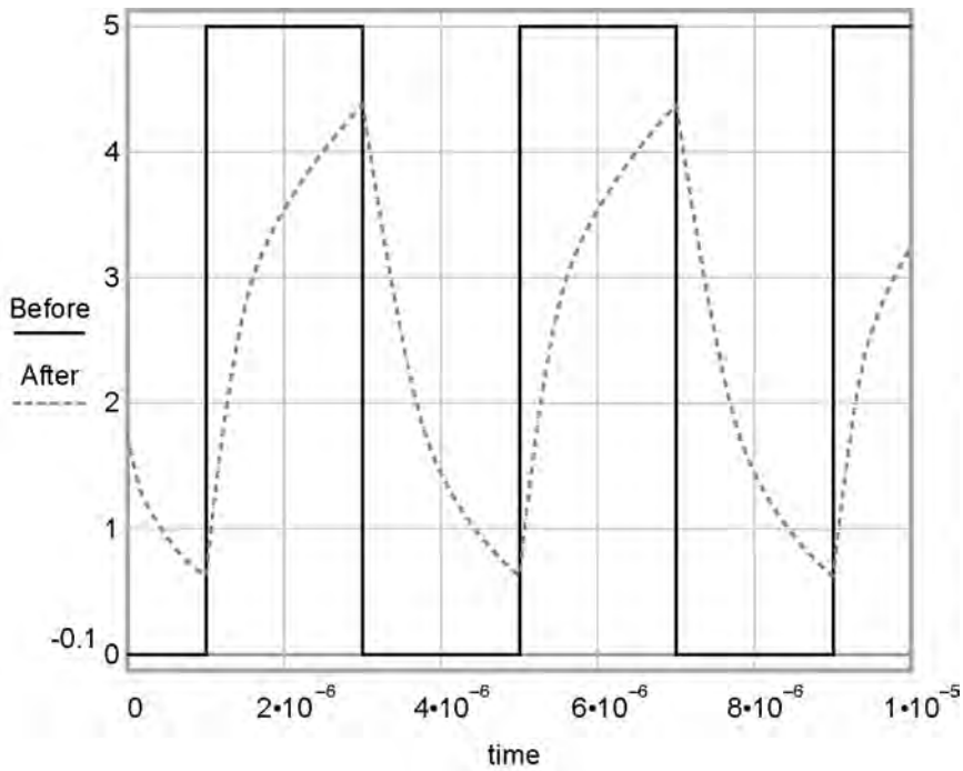
FIGURE 98: Amplitude reduction of pulse count waveform (before and after 1 \mu s \mu s time-constant filter)
