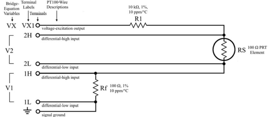
FIGURE 67: PT100 BrHalf4W() Four-Wire Half-Bridge Schematic
