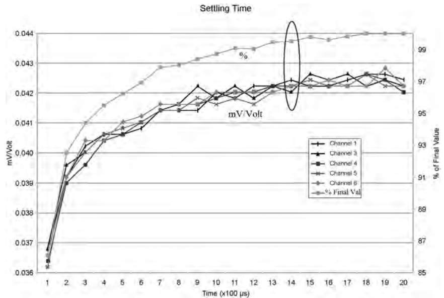
FIGURE 93: Settling Time for Pressure Transducer
