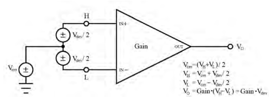
FIGURE 88: PGIA with Input Signal Decomposition
