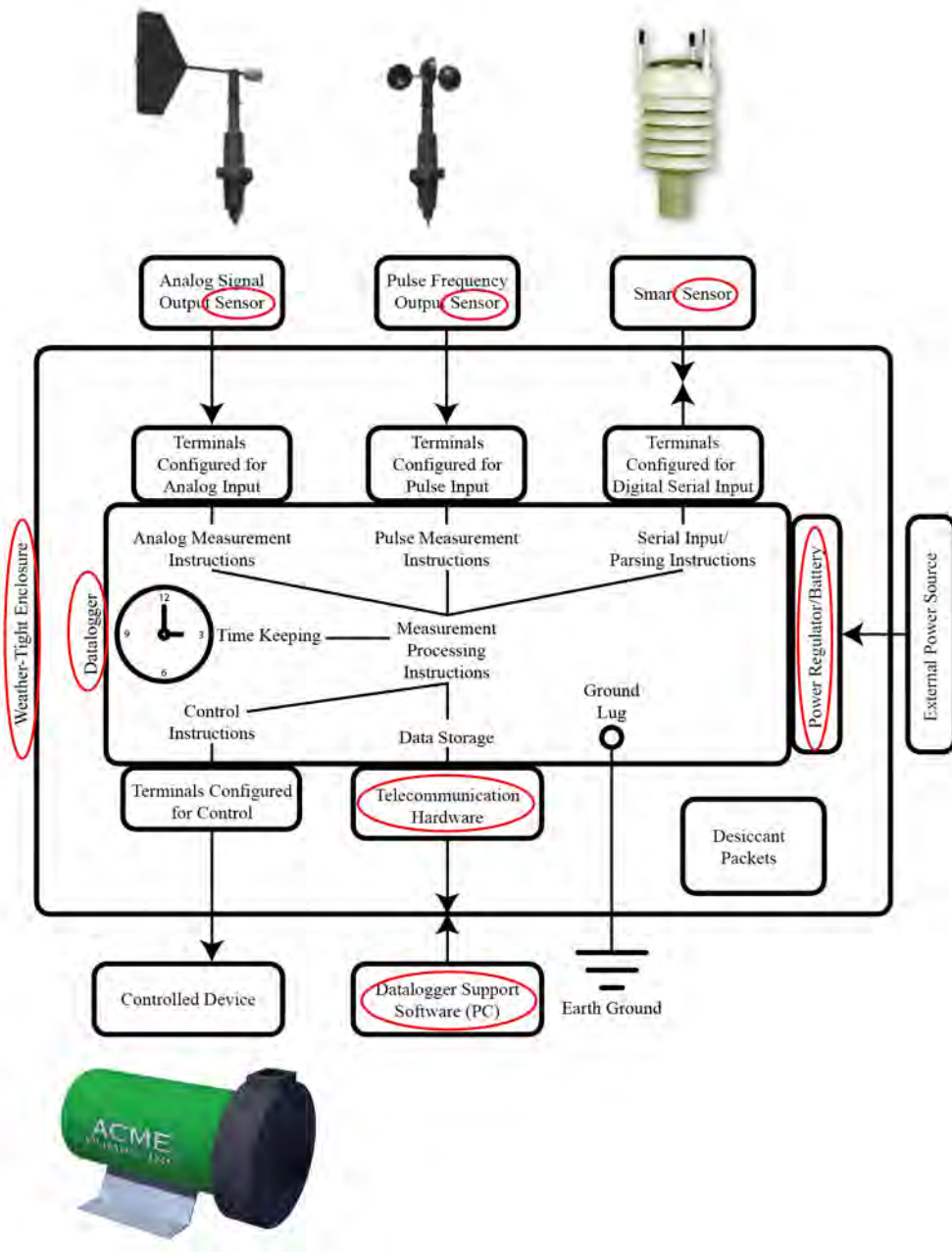
FIGURE 16: Data Acquisition System — Overview
