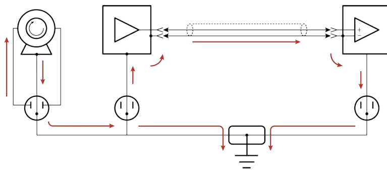
FIGURE 9-2. Leakage current (AC or DC) from nearby load
