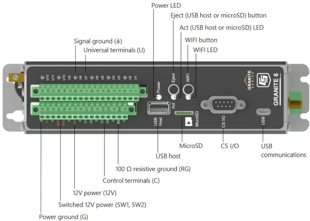
FIGURE 2-1. GRANITE 6 Wiring panel
